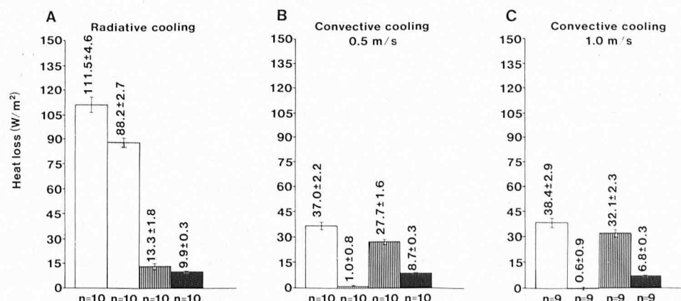
Figure 6. Total heat loss (white bars) and the radiative (light gray bars), convective (dark gray bars), and evaporative (black bars) heat loss fractions (mean \pm SEM) determined for the radiative cooling (A) and convective cooling by 0.5 ms -1 (B) and 1.0 ms -1 (C), respectively.
