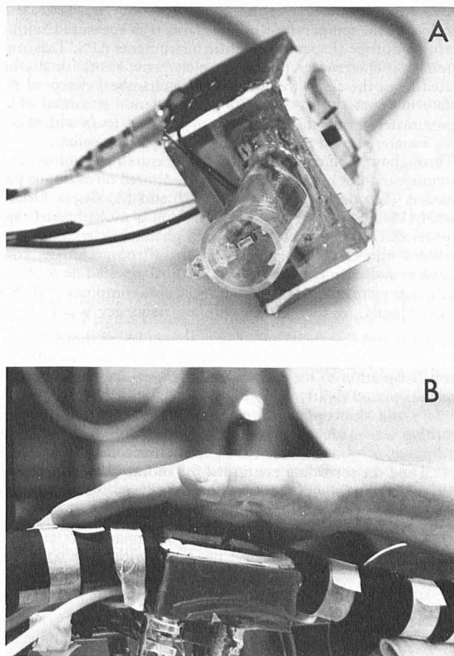
Figure 1. A, Microclimate chamber. B, Photograph showing the right hand and the microclimate chamber, to make clear the dimensional relations of the palm, the chamber, and the measuring probes.
